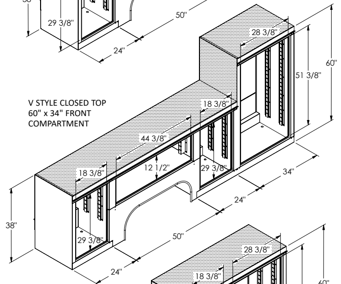
V STYLE 60" x 34" FRONT COMPARTMENT CLOSED TOP
