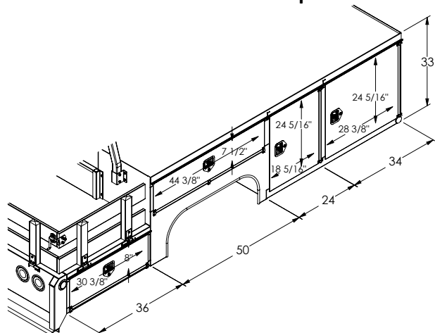
SEC-144-94-49-33-VD Closed Top
