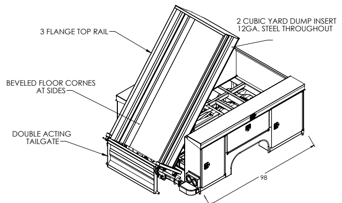
Dimensions for SB-98-79-49-38-VO 2 CUBIC YARD DUMP INSERT
