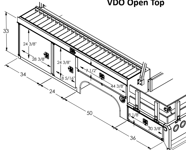
VDO Open Top
