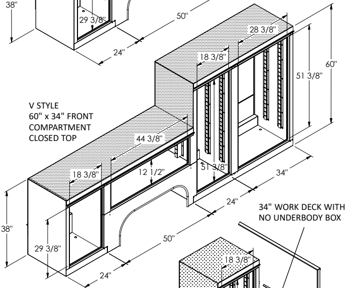
V STYLE CLOSED TOP
