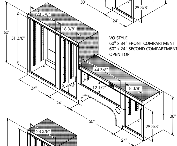
VO STYLE 60" x 34" FRONT COMPARTMENT WITH OPEN TOP
